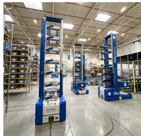
INTRABOT PICKER
